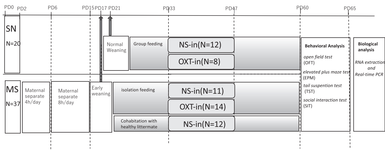
Figure 1. Experimental design
