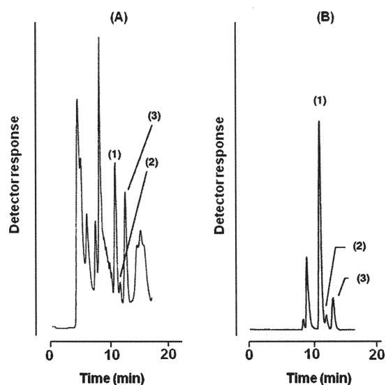
Figure 1. Chromatograms detected at 391 nm (A) and at 600 nm (B), which were obtained with urine spiked with PQ, DQ and IS (5 \mu\text{g}/\text{ml} ). Peaks: 1, PQ; 2, DQ; 3, IS; others, endogenous compounds.
