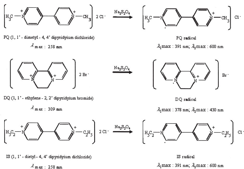
Figure 2. General scheme of the radicals from PQ, DQ, and IS by reduction with alkaline sodium hydrosulfite solution.
